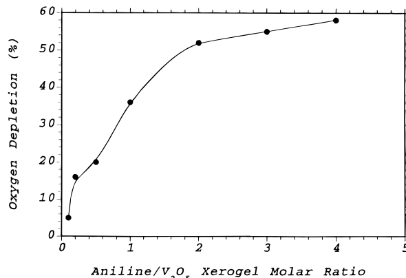
Figure 5. Oxygen consumption versus aniline/ V_2O_5 ratio. (At 0% consumption, the aqueous solution is saturated with oxygen.) Data taken at t = 15 min.
